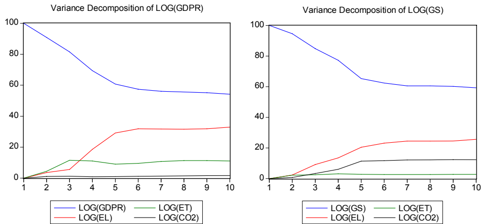
Figure A4. Relative variance contribution for real GDP growth and genuine savings rates
