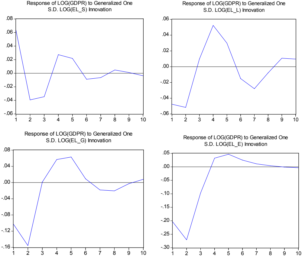
Figure A2. Responses of real GDP growth rates to impulses from four types of energy elasticities
