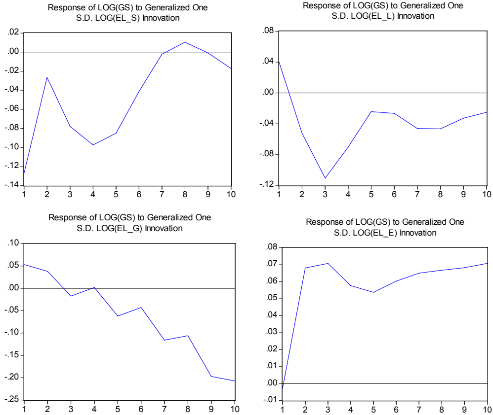
Figure A3. Responses of genuine savings rates to impulses from four types of energy elasticities
